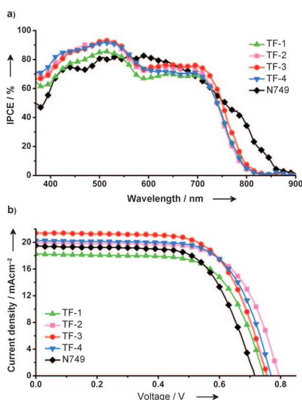
Figure 3. a) Photon-to-current action spectra and b) current–voltage characteristics of solar cells sensitized with various TF dyes and N749.
