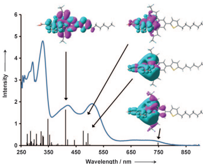
Figure 2. Experimental absorption spectrum of TF-2 sensitizer in DMF and the associated calculated spectrum. Black bars represent the computed vertical electronic excitations intensities ( f ) by TD-DFT method. The electron-hole density plots are shown for the selected electronic transitions at 412, 476, 493, and 748 nm, for which hole and excited electron densities are represented in pink and cyan, respectively.
