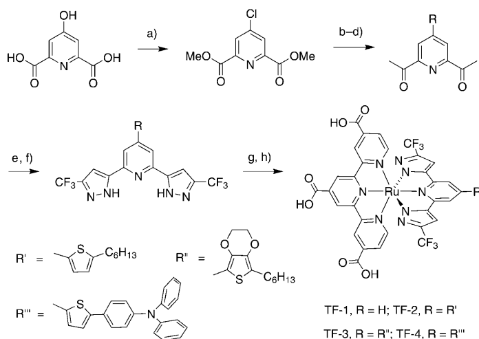
Scheme 2. Synthetic route to the Ru II sensitizers TF-1–TF-4. Reagents and conditions: a) PCl 5 , CHCl 3 , MeOH; b) EtOAc, NaOEt, reflux; c) HCl (aq) , reflux; d) Suzuki or Stille coupling, [Pd(PPh 3 ) 4 ]; e) CF 3 CO 2 Et, NaOEt, THF, reflux; f) N 2 H 4 , EtOH, reflux; g) [Ru(tectpy)Cl 3 ], EtOH, reflux; h) NaOH, acetone/H 2 O, acidification.
