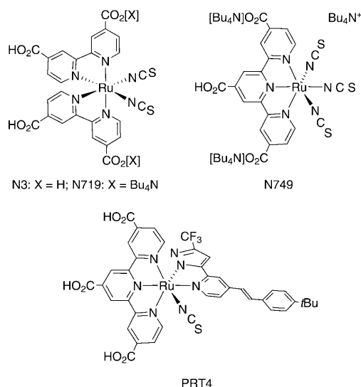
Scheme 1. Ru II sensitizers N3, N719, N749, and PRT4.
